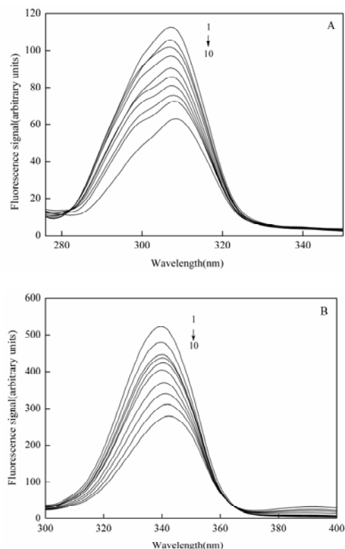
Figure 5. Fluorescence spectrum of CFS-trypsin systems ( T = 303 \text{ K} ) (A) \Delta\lambda=15\text{nm} ; (B) \Delta\lambda=60\text{nm} .
