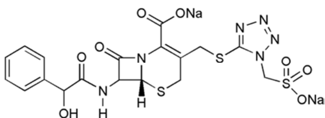
Figure 1. Chemical structure of Cefonicid Sodium.
