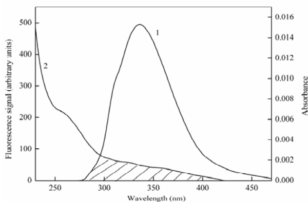
Figure 6. Overlap of the fluorescence spectrum of trypsin ( \lambda_{ex}=280\text{nm} ) (1) and the absorption spectrum of CFS (2) ( T = 303\text{K} ), C_{CFS} = C_{\text{Trypsin}} = 4.0 \times 10^{-6} \text{mol/L} .
